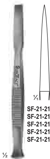
SF-21-213 - SF-21-217 Osteotome 140 mm
