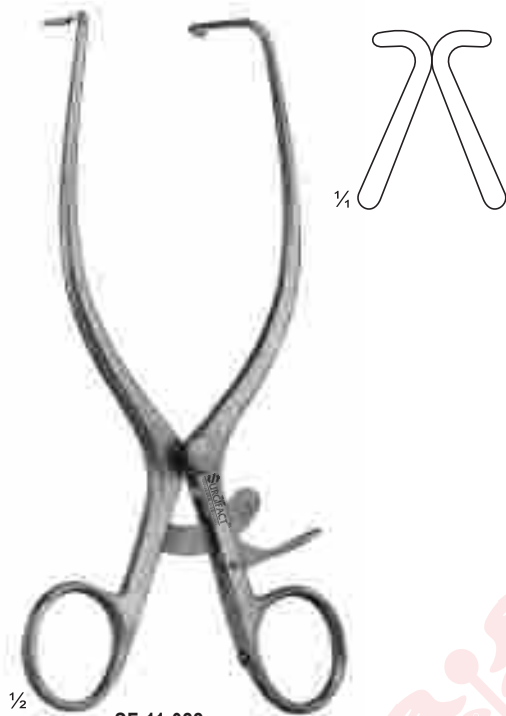
SF-11-022 JACKSON BURROWS Retractor, blunt 185 mm
